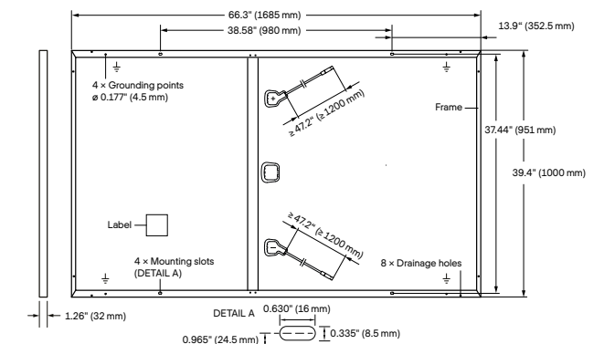
Fig. 2: External dimensions (in inch (mm)) and components for Q.PEAK DUO-G5.1, Q.PLUS DUO-G5.1, Q.PEAK DUO-G5.3 and Q.PLUS DUO-G5.3
