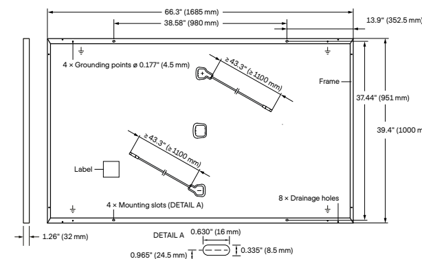
Fig. 1: External dimensions (in inch (mm)) and components for Q.PEAK DUO-G5, Q.PEAK DUO BLK-G5, Q.PLUS DUO-G5, Q.PLUS DUO BFR-G5, Q.PEAK DUO-G5.2, Q.PEAK DUO BLK-G5.2, Q.PLUS DUO-G5.2, Q.PLUS DUO BFR-G5.2
