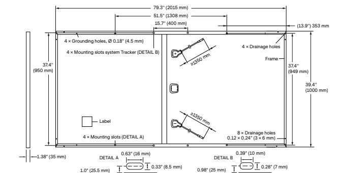
Fig. 2: External dimensions (in inch (mm)) and components for Q.PEAK DUO L-G5.1, Q.PEAK DUO L-G5.2, Q.PLUS DUO L-G5.1 and Q.PLUS DUO L-G5.2
