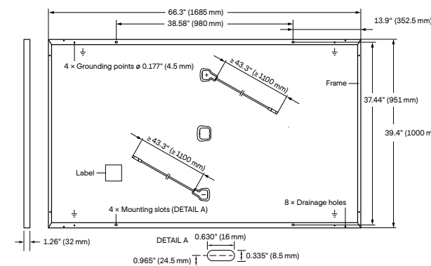
Fig. 1: External dimensions (in inch (mm)) and components for Q.PEAK DUO-G7, Q.PEAK DUO BLK-G7, Q.PEAK DUO-G7.2 and Q.PEAK DUO BLK-G7.2
