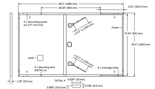
Fig. 2: External dimensions (in inch (mm)) and components for Q.PEAK DUO-G7.1 and Q.PEAK DUO-G7.3
