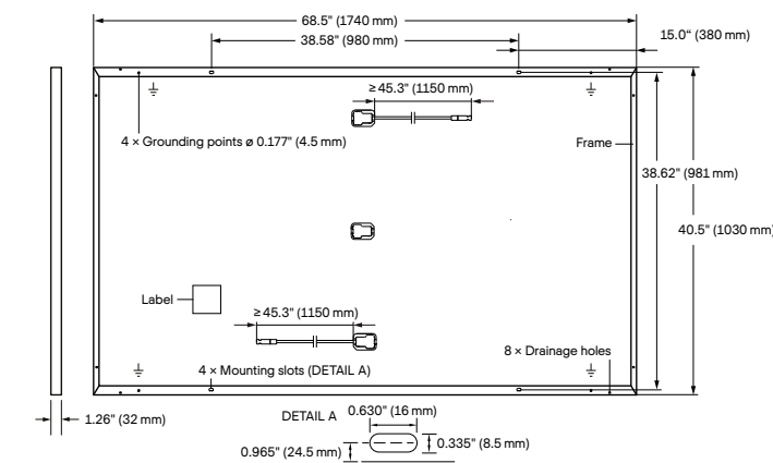
Fig. 1: External dimensions (in inch (mm)) and components for Q.PEAK DUO-G8, Q.PEAK DUO BLK-G8, Q.PEAK DUO-G8+ and Q.PEAK DUO BLK-G8+
