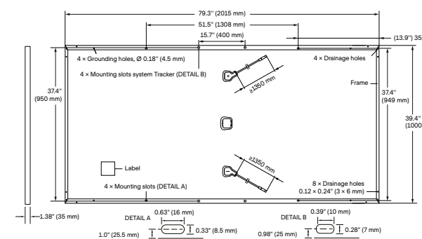
Fig. 1: External dimensions (in inch (mm)) and components for Q.PEAK DUO L-G7 and Q.PEAK DUO L-G7.3
