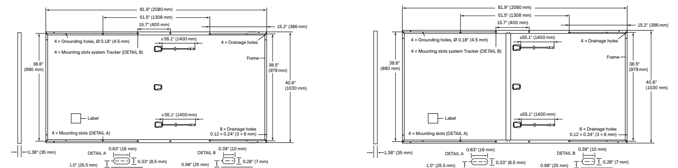
Fig. 1: External dimensions (in inch (mm)) and components for Q.PEAK DUO L-G8 and Q.PEAK DUO L-G8.3
