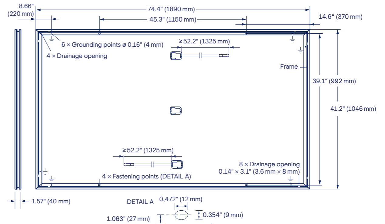
Fig. 1: External dimensions (in inch (mm)) and components for Q.PEAK DUO BLK ML-G10+/TS
